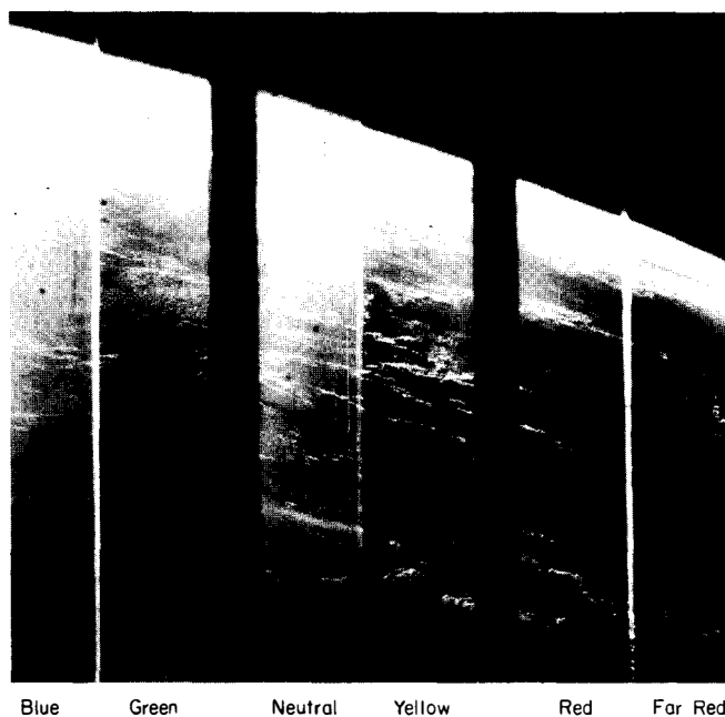
FIGURE 52. —For the Mercury-Atlas 8 experiment a fixed-band set of filters was incorporated in the dark slide. In this continuous picture of the surface of the Earth, the separate elements are recorded in the different spectral bands. Note the displacement in the horizon which was a significant target of this experiment. The picture was taken by Walter Schirra and shows the Atlantic southeast of Brazil.
