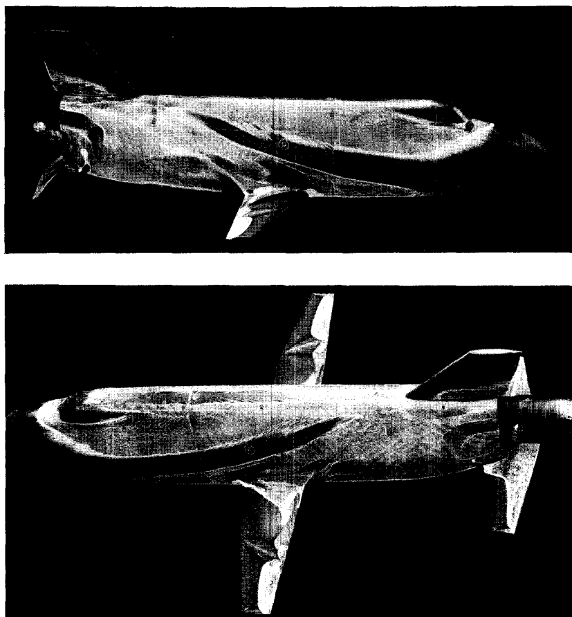
FIGURE 23.—These photographs show opposite sides of a flight model with surface air patterns visualized by the use of oil-flow techniques. The viscous oil visible in pictures retains its position on cooling, allowing the detailed photographs to be made after the air flow has been terminated.
