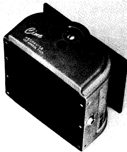
FIGURE 5.—A variation of the device shown in figure 4 was developed for the Gemini program, with a plate attached for storing the magazines. After experimenting with a silver finish, the decision was made to continue with a black finish until the lunar landing.
