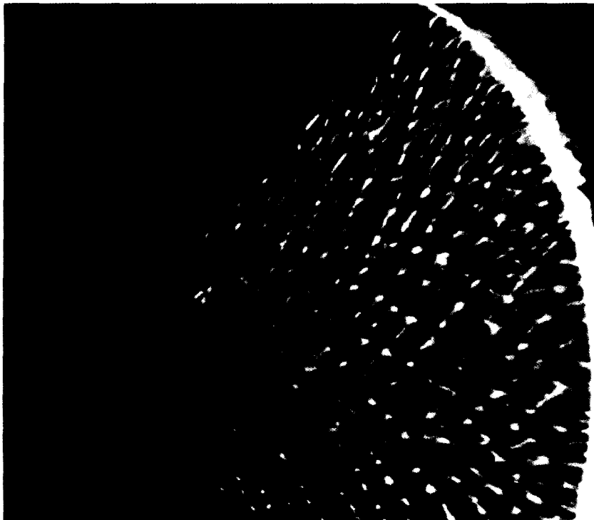
A closeup of patterns formed during ablation on a Lexan plastic model of a cone form. A sequence of pictures of this occurrence shows how the pattern forms as velocity increases and ablation develops.
