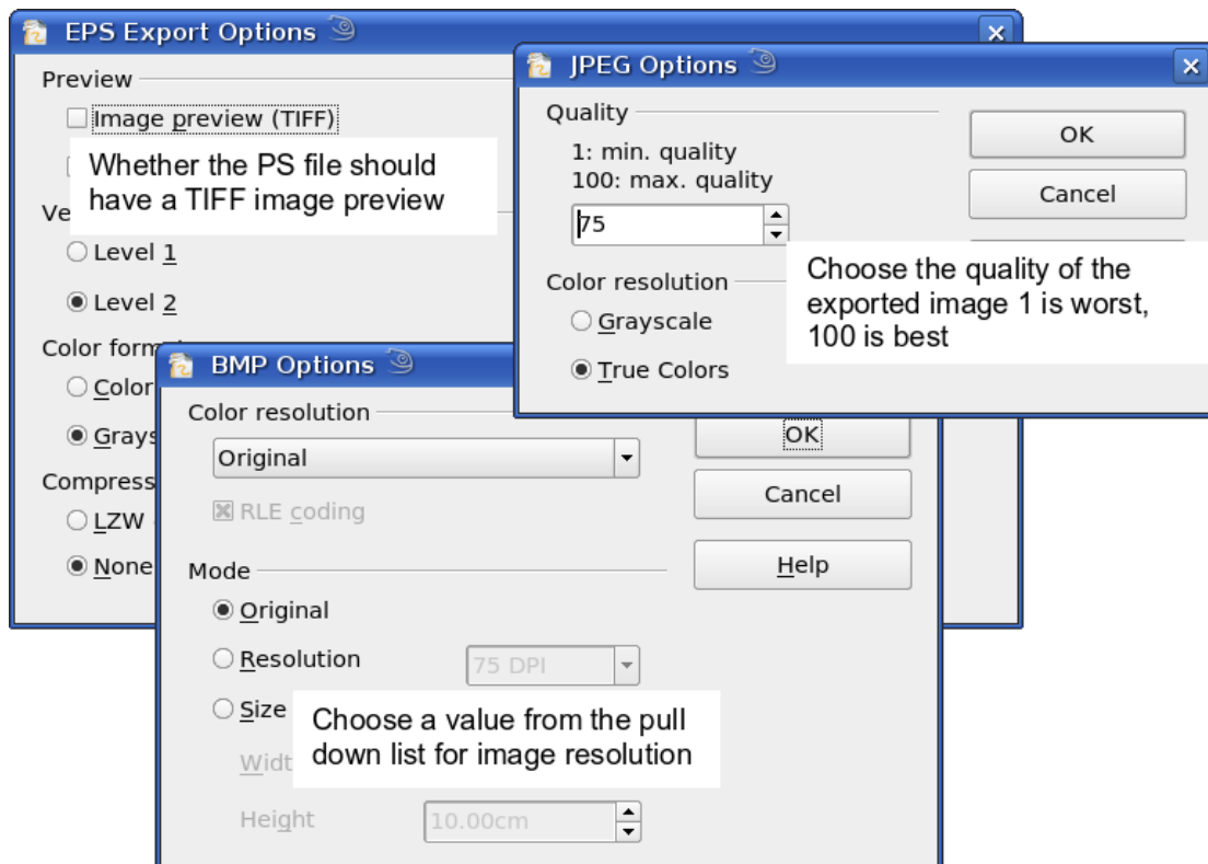
Figure 6: Adjusting format specific properties prior to export
