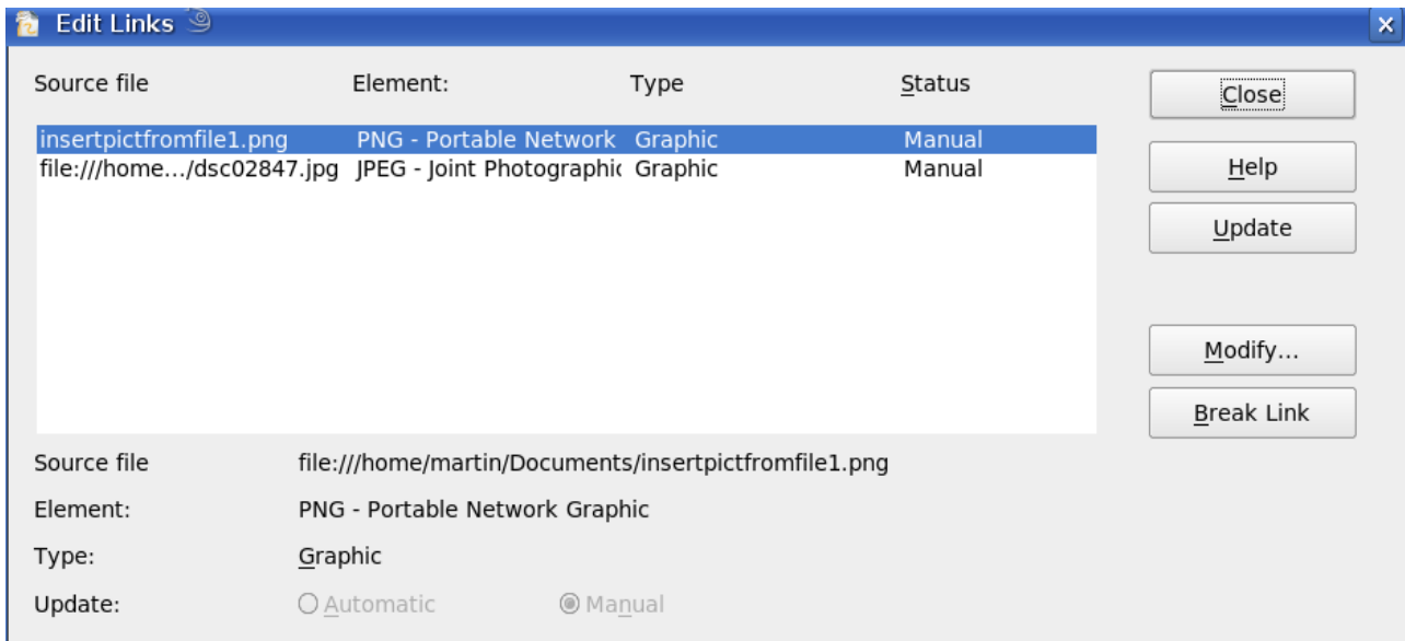
Figure 2: Editing links to documents
